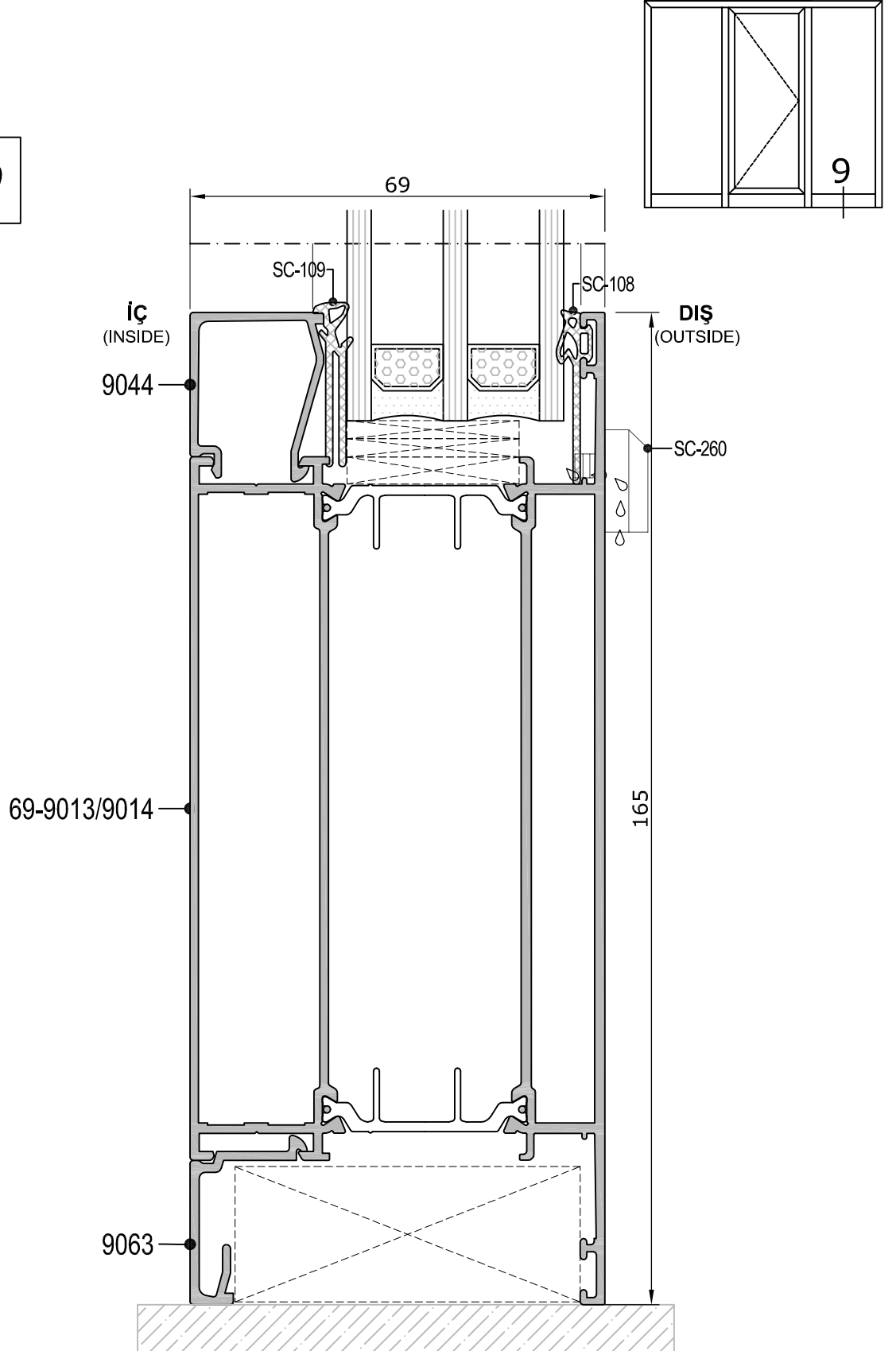
Detay Detail 9
