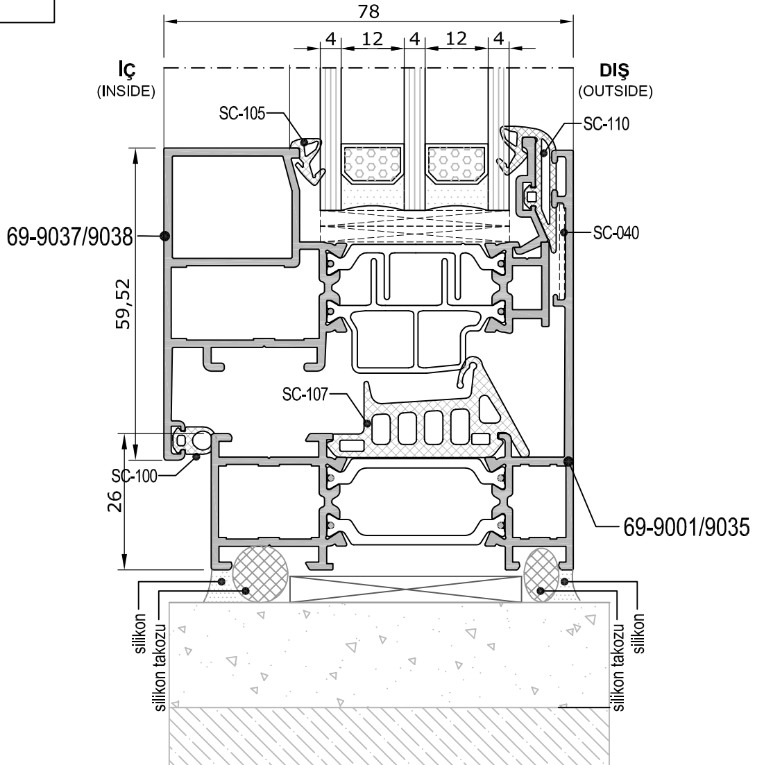
Detay Detail 22
