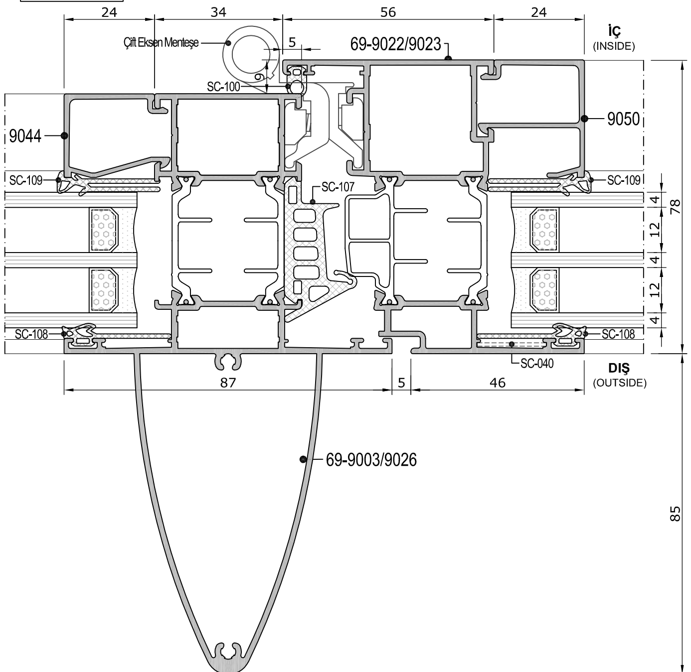
Detay 8 Detail
