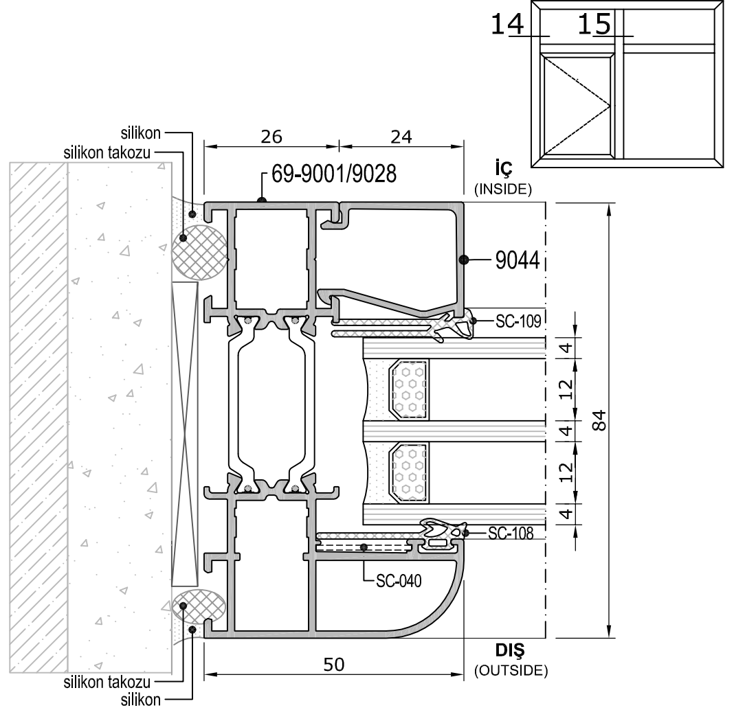
Detay Detail 14
