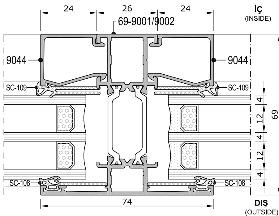
Detay Detail 2
