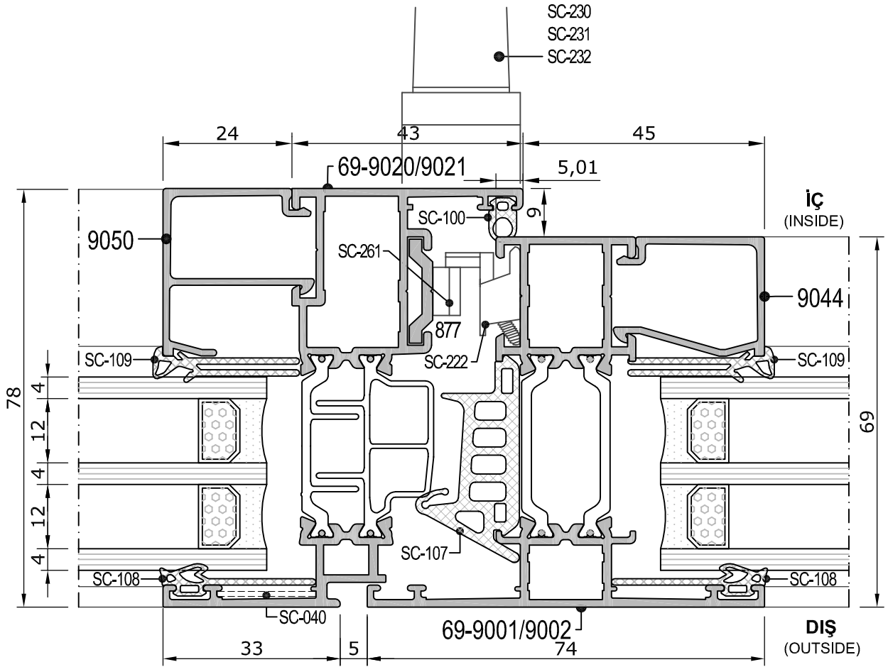
Detay Detail 4
