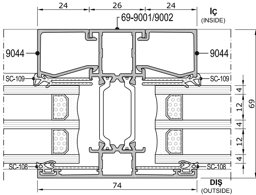
Detay Detail 15
