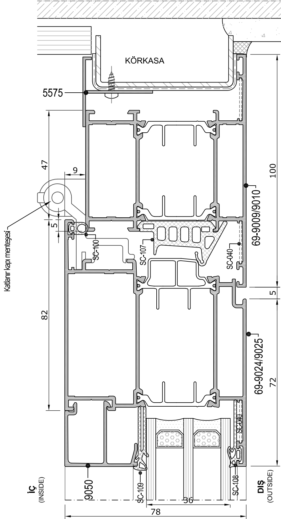
Detay 28 Detail
